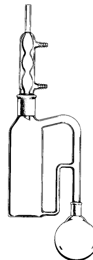
Continuous Liquid/Liquid
